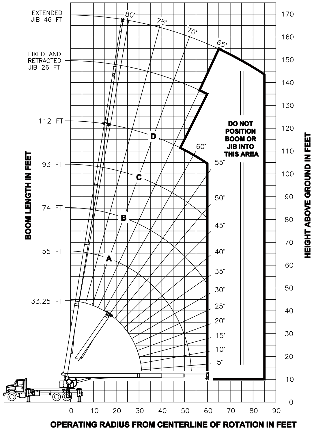
RANGE DIAGRAM - MID EXTEND OUTRIGGER CONFIGURATION -
